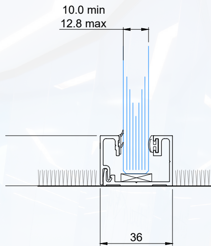
SINGLE GLAZED FLOOR TRACK 36mm x 25mm WITH CLIP-IN BEAD
