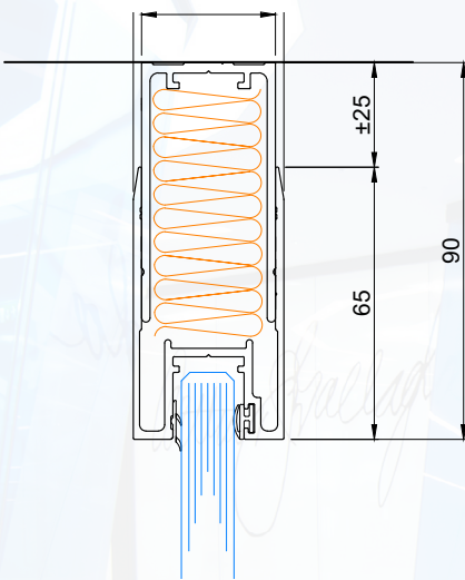
SINGLE GLAZED HEAD TRACK WITH INNER UPPER CHANNEL ± 25MM DEFLECTION
