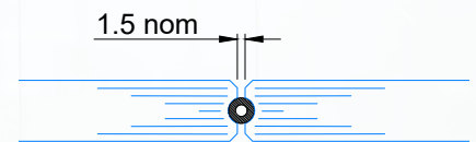
GLASS TO GLASS NEBULA™ PATENTED DRY JOINT
